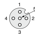
Socket connector pin arrangement A-coded (Normal key)
