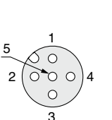
Plug connector pin arrangement A-coded (Normal key)
