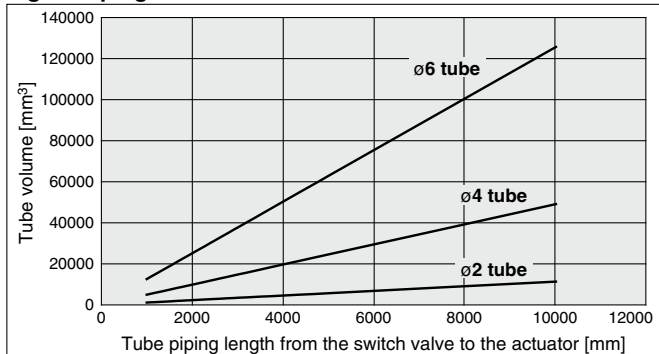
Fig. 2 Piping Volume Chart
