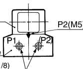
VEX3422 Internal pilot solenoid for subplate
