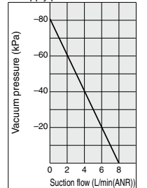
ZA07 Flow Characteristics Supply pressure: 0.45 MPa
