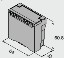
Existing model (Series EX120)
