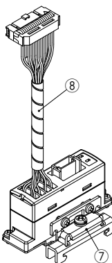
EX510-S□02A (Series SY, VQ)
