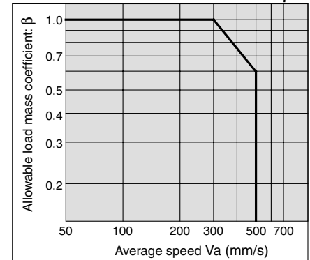
Graph (1) Allowable Load Mass Coefficient: \beta
