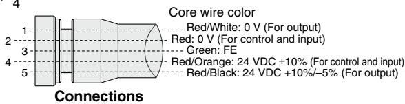
Socket pin arrangement
