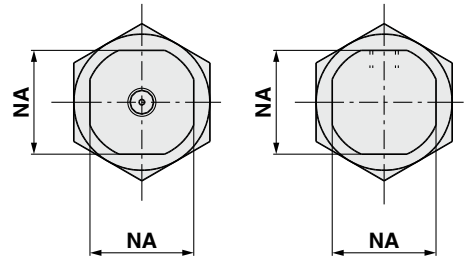
Head cover axial port Boss-cut/Basic Band mounting (B) Without magnet
