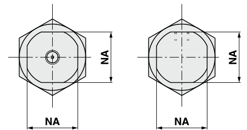
Head cover axial port
