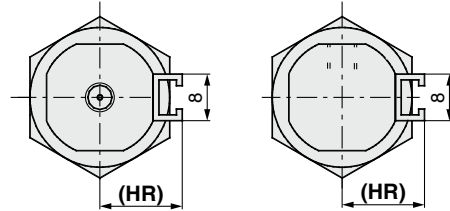
Head cover axial port Boss-cut/Basic Rail mounting (A)
