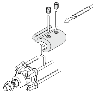
• Mounting example for D-A9□(V), M9□(V), M9□W(V), M9□A(V)
