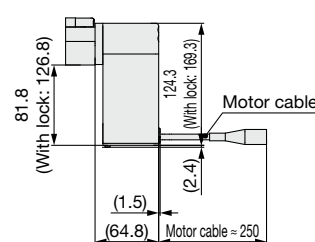
Motor mounting position: U
