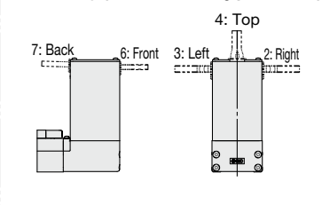
Cable Entry (Motor mounting position: T)
