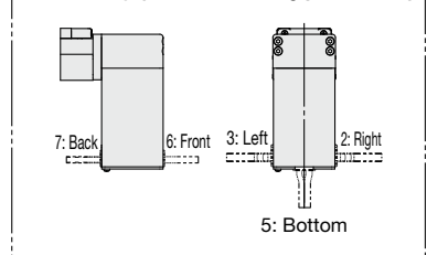
Cable Entry (Motor mounting position: U)
