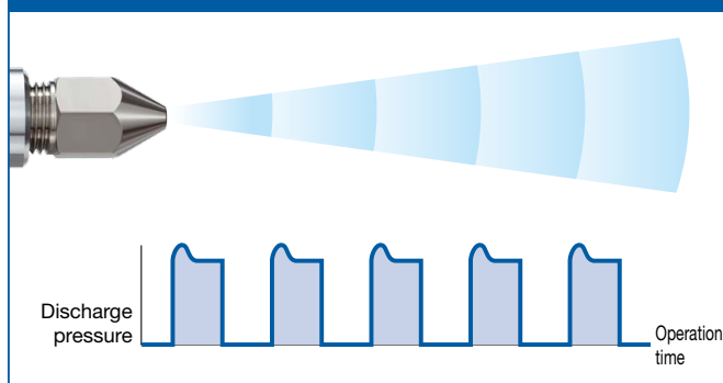
Pulse blow
