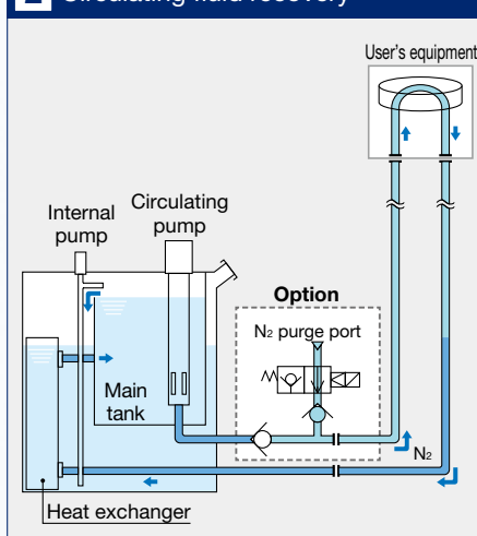
2 Circulating fluid recovery
