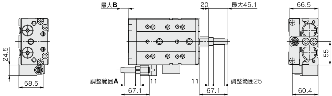
MXQ32-□□B,BS,BT-X2600 (mm)
