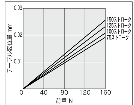
MXQ32-75,100,125,150-X2600
