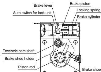
Locked condition (when air is exhausted.)
