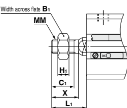
Rod End Male Thread
