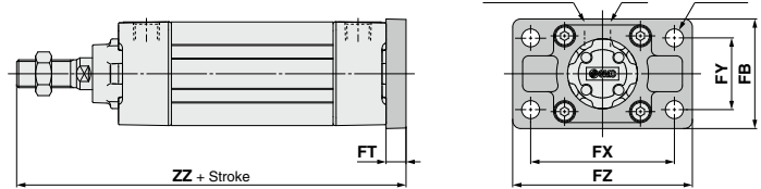
Head Flange
