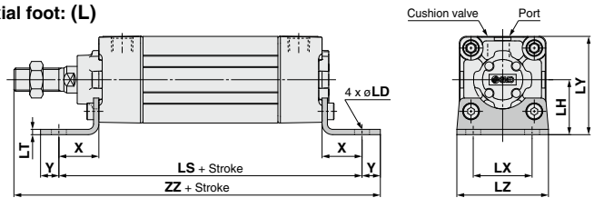
Axial Foot
