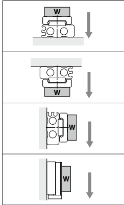
Fig. (3) Workpiece Mounting Coefficient: K
