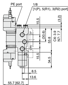
L-type plug connector (L)
