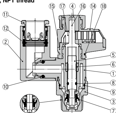
Meter-in
