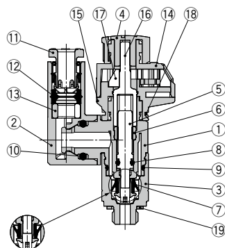
Meter-in
