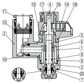
Meter-in
