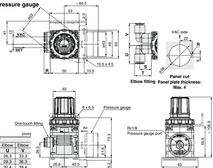
Fitting Part Dimensions
