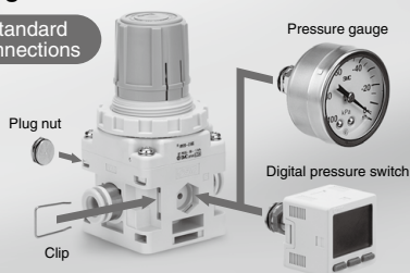
Single sided connections
