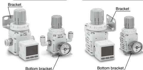
Standard connections
