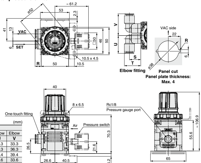
Fitting Part Dimensions
