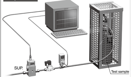
Proof pressure test ((Example) Tank)
